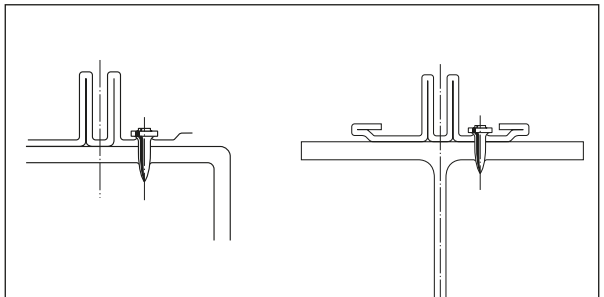
Fastening glass facade attachment profiles using the DX 450 (125%, 8 mm narrow access)
