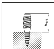
Nail standoff
